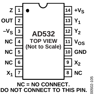
Figure 4. 14-Lead Side Brazed DIP (D-14)
