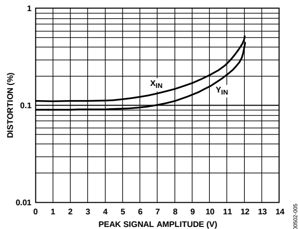
Figure 5. Distortion vs. Peak Signal Amplitude
