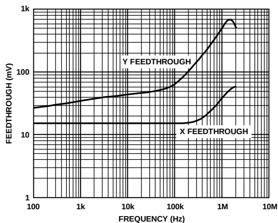
Figure 7. Feedthrough vs. Frequency
