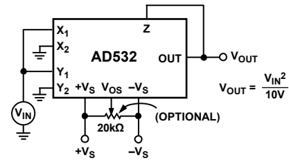
Figure 15. Squarer Connection
