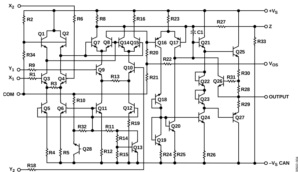
Figure 13. Schematic Diagram
