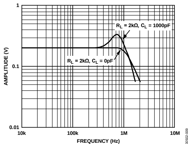
Figure 9. Frequency Response, Multiplying
