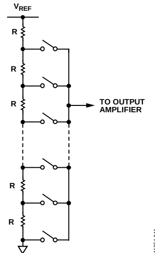
Figure 39. Resistor String Structure
