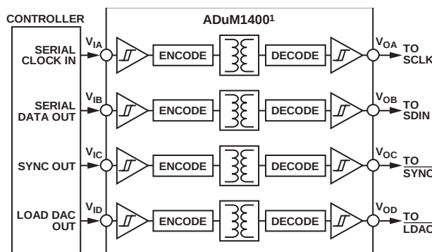
Figure 50. Isolated Interface
