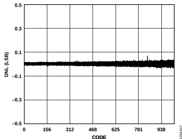
Figure 15. Differential Nonlinearity (DNL) vs. Code
