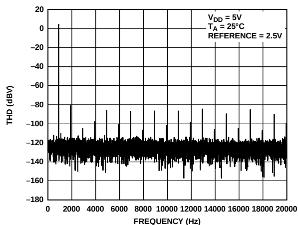
Figure 36. Total Harmonic Distortion at 1 kHz
