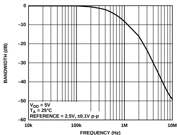
Figure 37. Multiplying Bandwidth, External Reference = 2.5 V, \pm 0.1 V p-p, 10 kHz to 10 MHz
