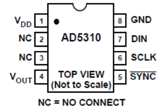
Figure 4. \mu SOIC
