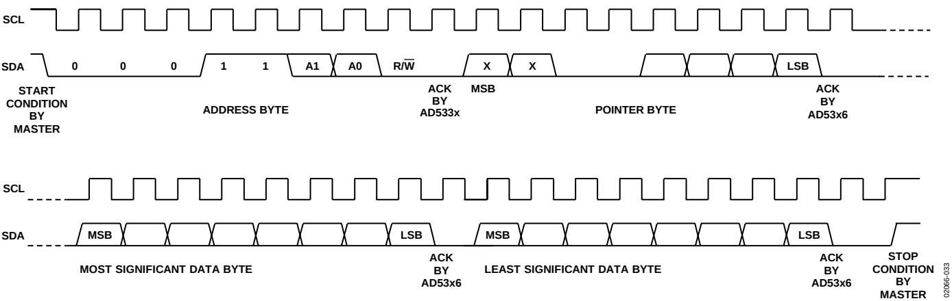
Figure 33. Write Sequence
