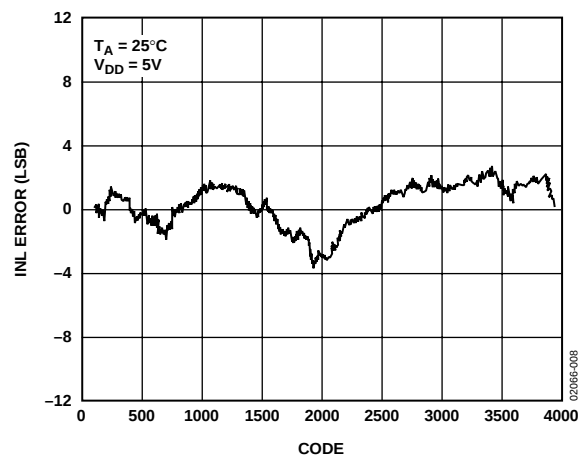
Figure 8. AD5326 INL
