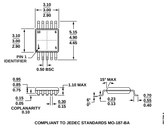
Figure 45. 10-Lead Mini Small Outline Package [MSOP] (RM-10)
