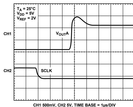
Figure 22. Exiting Power-Down to Midscale
