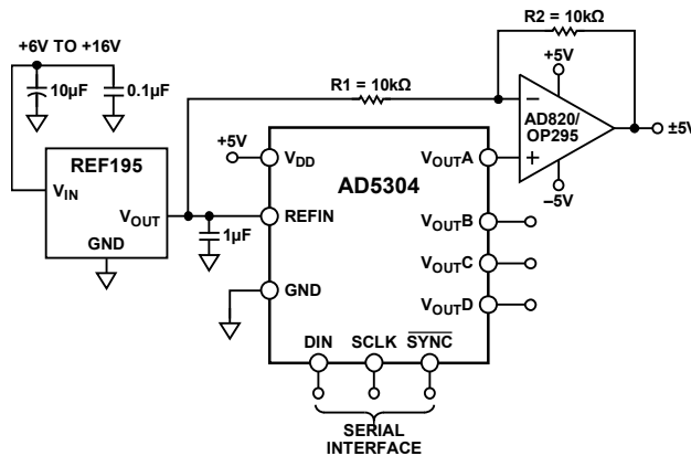
Figure 41. Bipolar Operation with the AD5304
