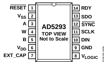
Figure 5. Pin Configuration
