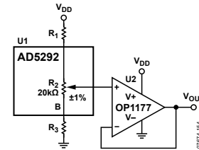
Figure 72. Optimizing Resolution
