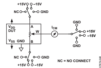
Figure 63. Common-Mode Leakage Current
