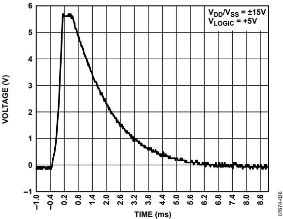
Figure 54. V_{EXT\_CAP} Waveform While Reading Fuse or Calibration
