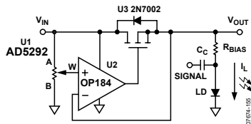
Figure 71. Programmable Boosted Voltage Source
