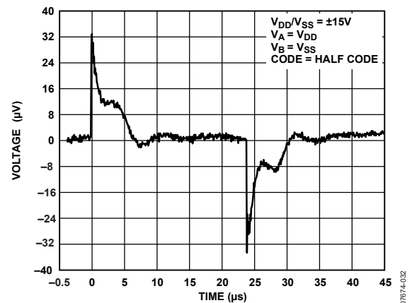
Figure 53. Digital Feedthrough
