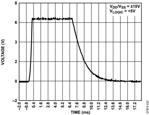
Figure 55. V_{EXT\_CAP} Waveform While Writing Fuse
