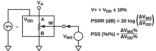
Figure 35. Power Supply Sensitivity (PSS, PSRR)
