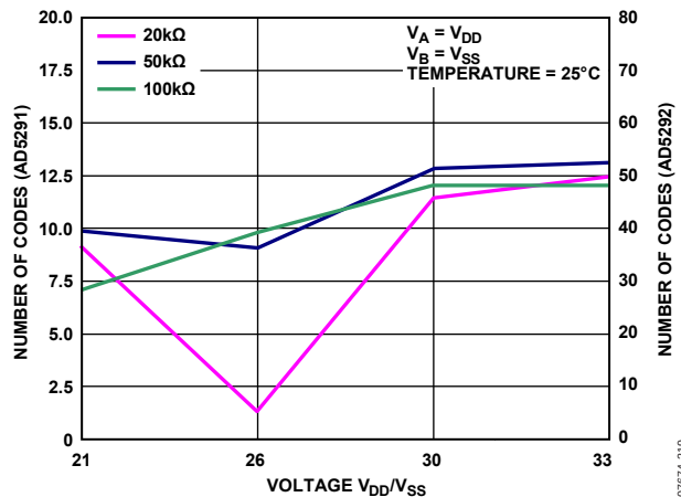
Figure 57. Code Range &gt; 1% R-Tolerance Error vs. Voltage
