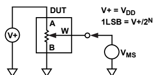
Figure 59. Potentiometer Divider Nonlinearity Error (INL, DNL)
