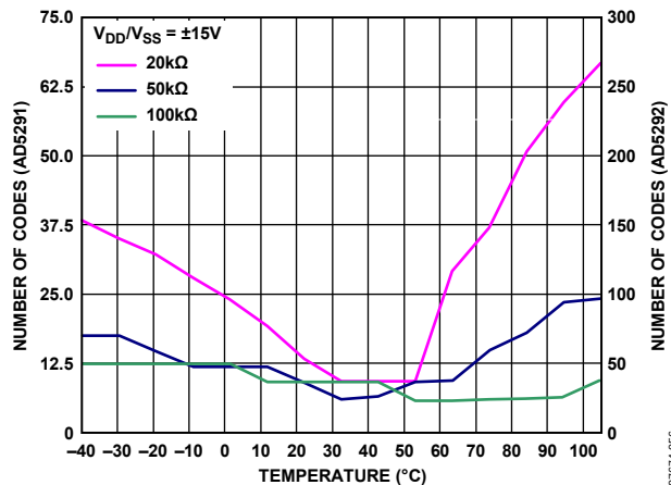
Figure 56. Code Range &gt; 1% R-Tolerance Error vs. Temperature
