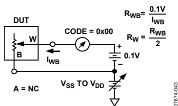
Figure 60. Wiper Resistance
