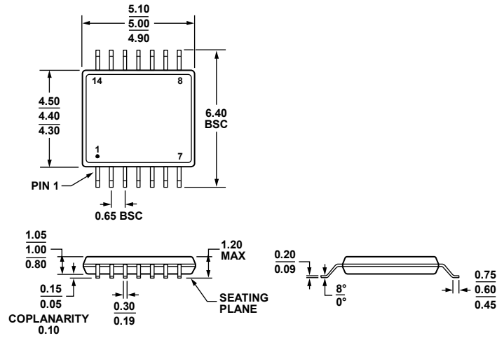
Figure 76. 14-Lead Thin Shrink Small Outline Package [TSSOP] (RU-14) Dimensions shown in millimeters
