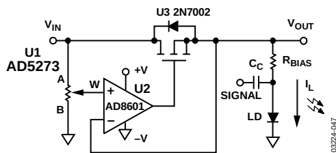
Figure 44. Programmable Booster Voltage Source
