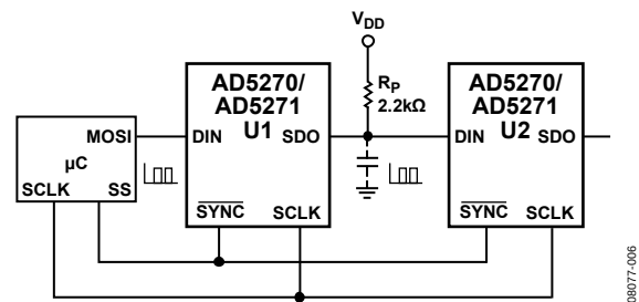
Figure 44. Daisy-Chain Configuration Using SDO
