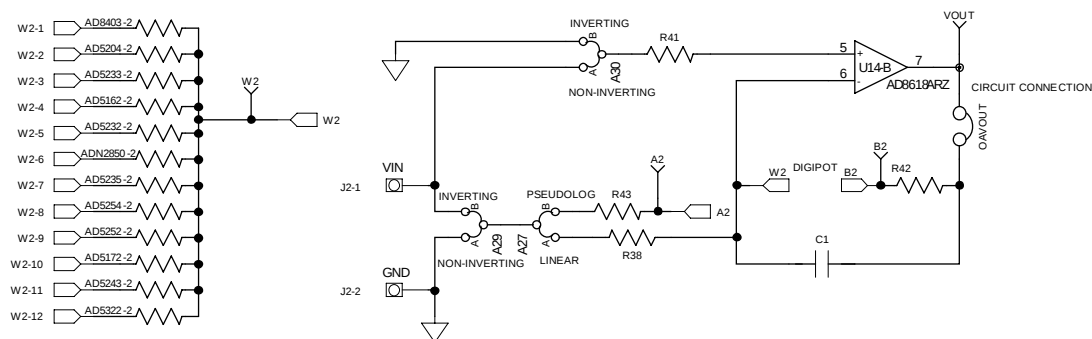
Figure 12. Schematic of Multiboard RDAC Circuits
