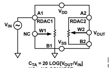
Figure 34. Analog Crosstalk
