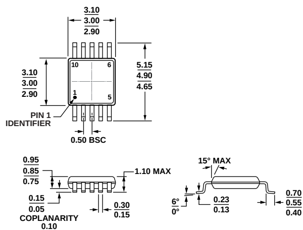
COMPLIANT TO JEDEC STANDARDS MO-187-BA Figure 15. 10-Lead Mini Small Outline Package [MSOP] (RM-10) Dimensions shown in millimeters
