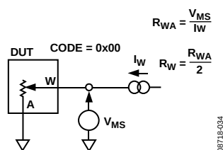
Figure 22. Wiper Resistance
