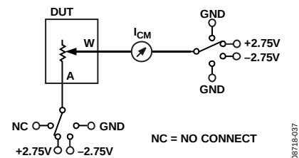
Figure 25. Common Leakage Current
