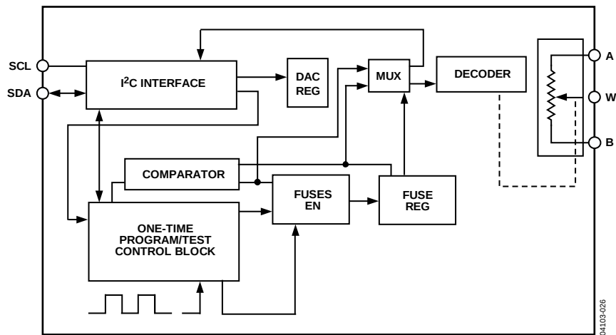
Figure 39. Detailed Functional Block Diagram
