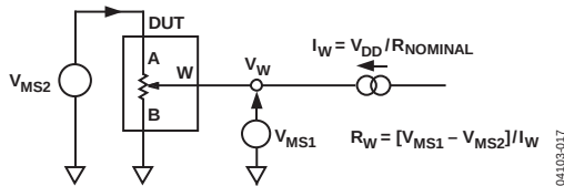
Figure 33. Wiper Resistance
