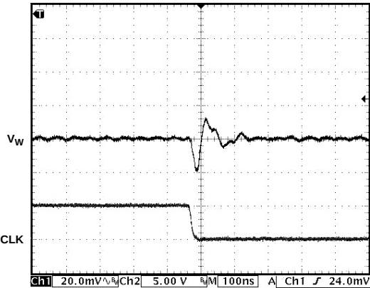
Figure 22. Digital Feedthrough
