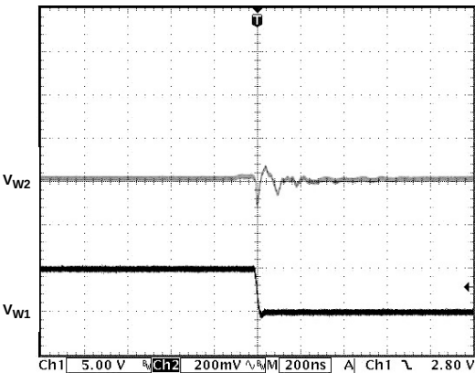
Figure 23. Digital Crosstalk
