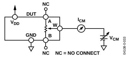
Figure 32. Test Circuit for Common-Mode Leakage Current
