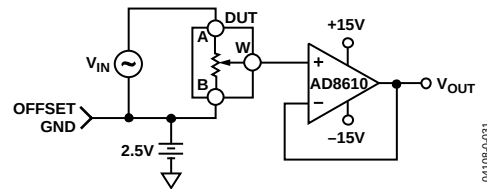
Figure 31. Test Circuit for Gain vs. Frequency
