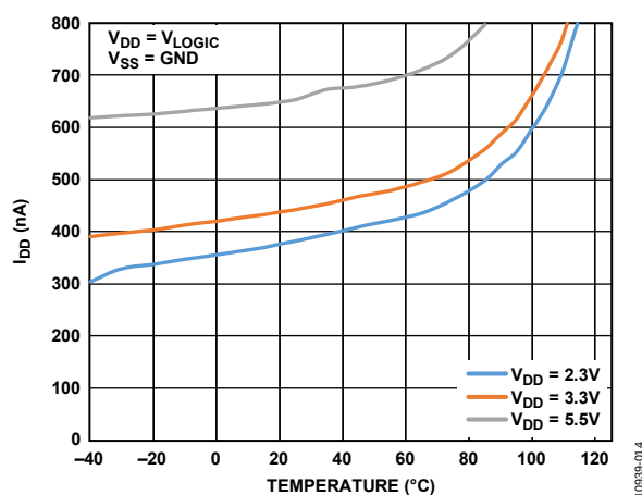
Figure 14. I_{\text{DD}} vs. Temperature
