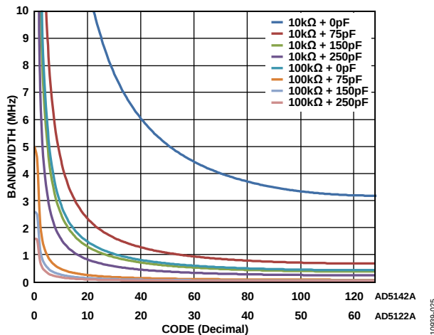
Figure 26. Maximum Bandwidth vs. Code and Net Capacitance
