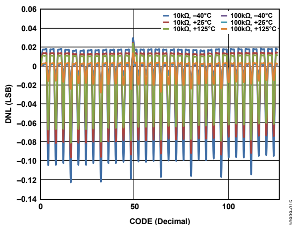
Figure 16. DNL vs. Code (AD5122A)
