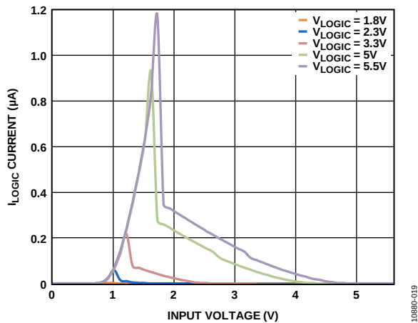
Figure 20. I_{\text{LOGIC}} Current vs. Digital Input Voltage
