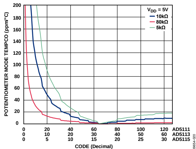
Figure 19. Potentiometer Mode Tempco ( (\Delta V_w/V_w)/\Delta T \times 10^6 ) vs. Code
