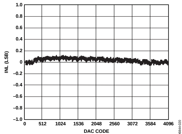
Figure 7. AD5045 INL
