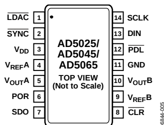
Figure 5. Pin Configuration
