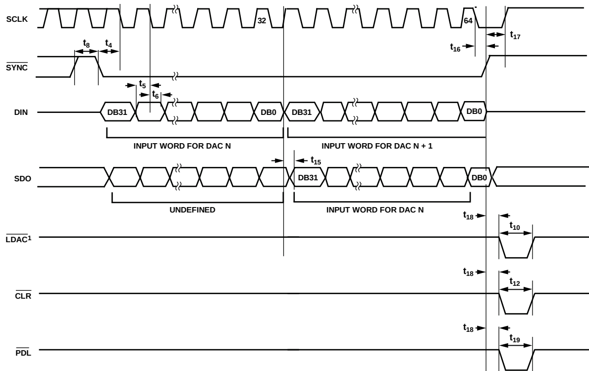
Figure 4. Daisy-Chain Timing Diagram
