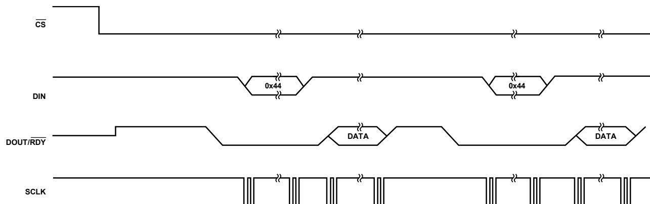
Figure 44. SPI Communication in Continuous Conversion Mode
