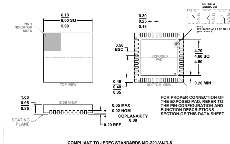
Figure 47. 40-Lead Lead Frame Chip Scale Package [LFCSP] 6 mm × 6 mm Body and 0.95 mm Package Height (CP-40-15)
