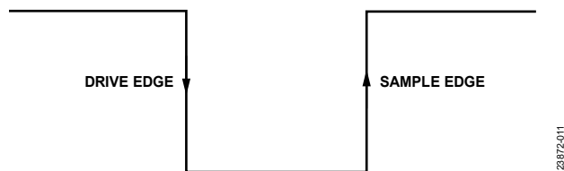
Figure 21. SPI Mode 3 SCLK Edges
