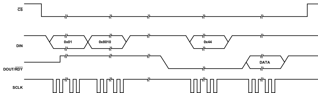
Figure 46. SPI Communication in Single Conversion Mode
