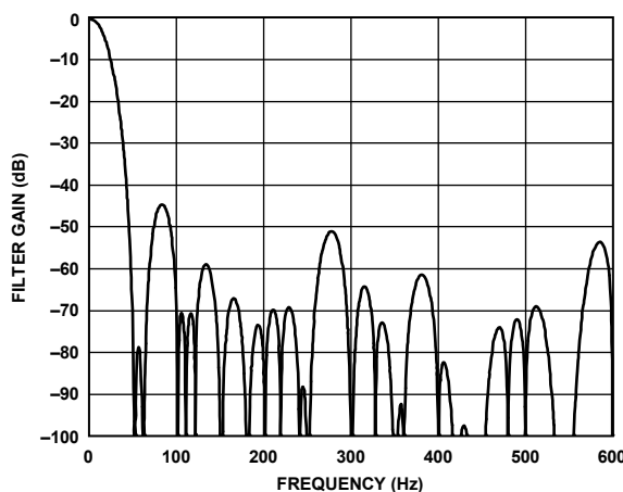
Figure 42. 16.667 SPS ODR, 60 ms Settling Time
