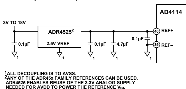
Figure 29. ADR4525 Connected to AD4114 REF+ and REF– Pins
