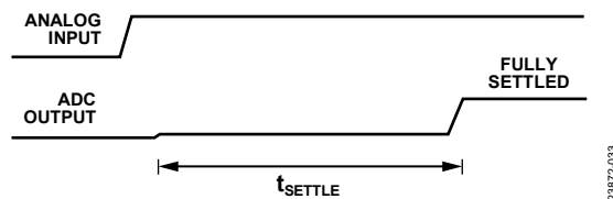
Figure 35. Step Input with Single Cycle Settling
