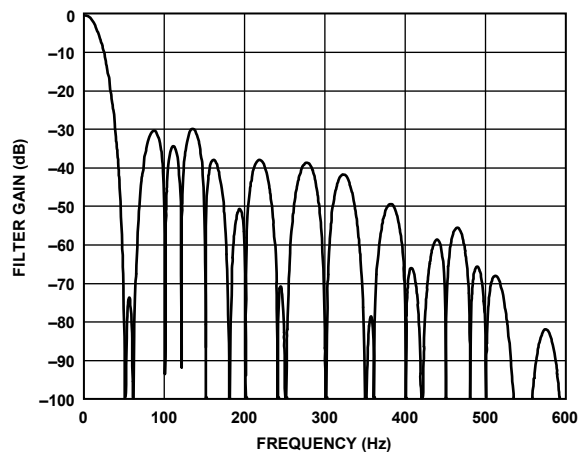
Figure 38. 20 SPS ODR, 50 ms Settling Time
