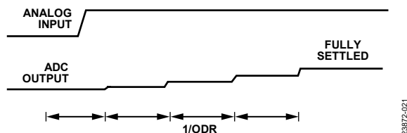
Figure 34. Step Input Without Single Cycle Settling
