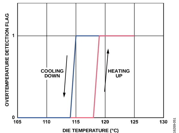
Figure 51. Overtemperature Detection
