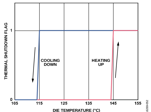
Figure 52. Thermal Shutdown
