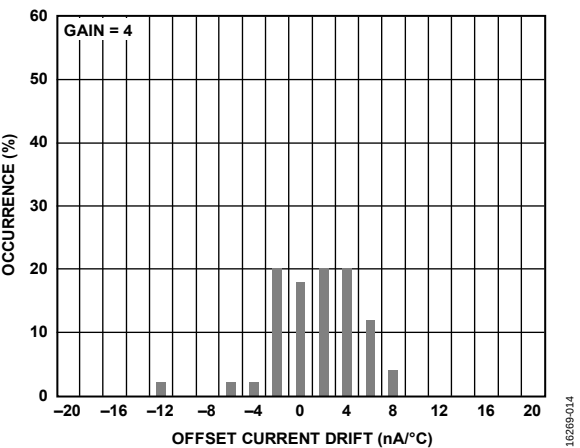
Figure 14. Current Mode, Offset Current Drift Distribution (Gain = 4)
