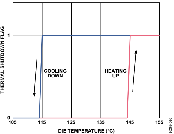
Figure 16. Thermal Shutdown
