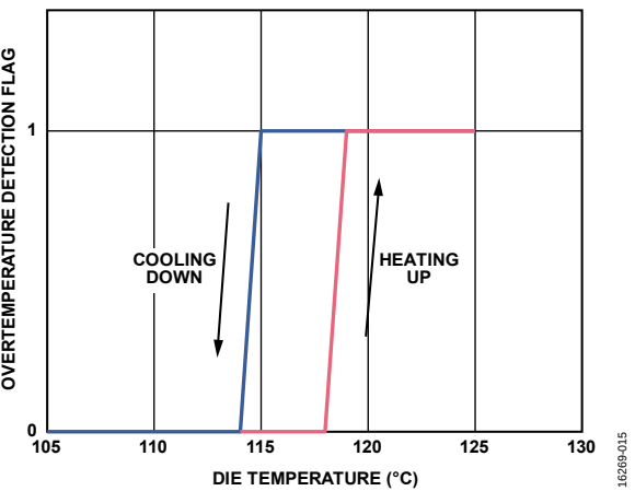
Figure 15. Overtemperature Detection
