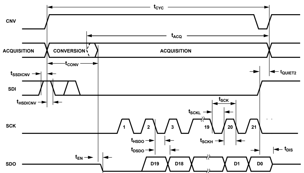
Figure 64. \overline{\text{CS}} Mode, 4-Wire with the Busy Indicator Serial Interface Timing Diagram (Status Bits Not Shown)
