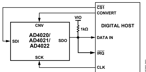
Figure 63. \overline{\text{CS}} Mode, 4-Wire with Busy Indicator Connection Diagram
