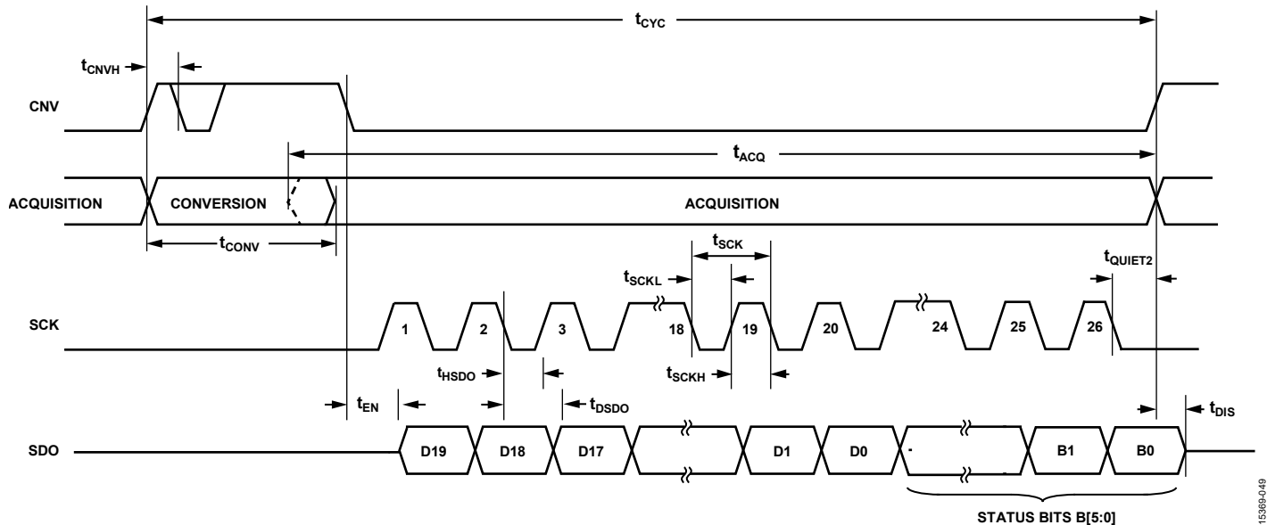
Figure 52. \overline{\text{CS}} Mode, 3-Wire Without Busy Indicator Serial Interface Timing Diagram Including Status Bits
