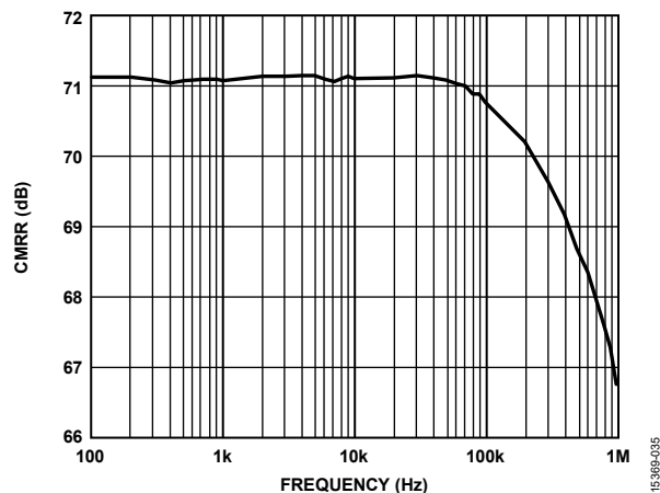
Figure 32. Common-Mode Rejection Ratio (CMRR) vs. Frequency
