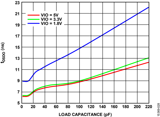
Figure 37. t_{DSO} vs. Load Capacitance
