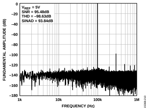
Figure 13. 100 kHz, -0.5 dBFS Input Tone FFT, Wide View
