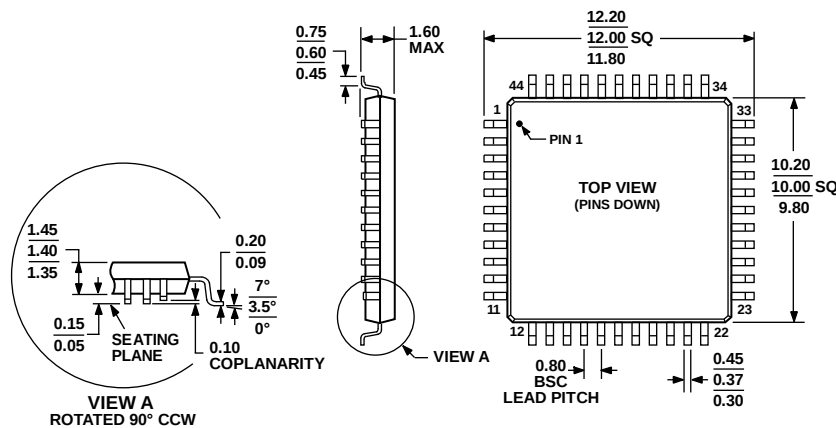
Figure 17. 44-Lead Low Profile Quad Flat Package [LQFP] (ST-44-1) Dimensions shown in millimeters
