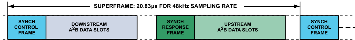
Figure 3. A²B Superframe
