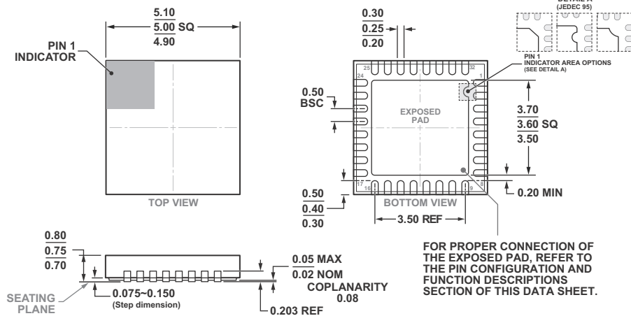
Figure 39. 32-Lead Lead Frame Chip Scale Package [LFCSP_SS] 5 mm x 5 mm Body, With Side Solderable Leads (CS-32-2) Dimensions shown in millimeters
