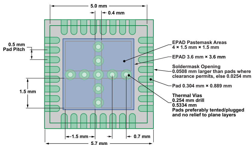
Figure 38. Transceiver Footprint
