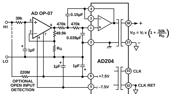
Figure 17. Input Amplifier & Filter for Sensor Signals
