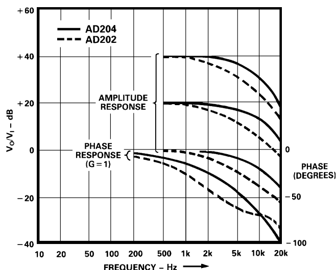
Figure 11. Frequency Response at Several Gains
