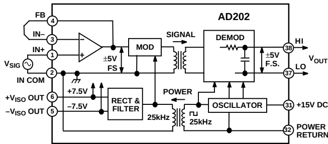
Figure 1a. AD202 Functional Block Diagram
