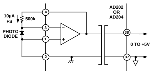
Figure 22. Photodiode Amplifier
