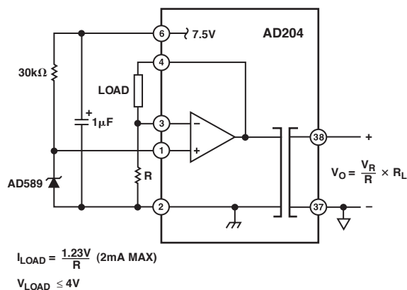
Figure 21. Floating Current Source
