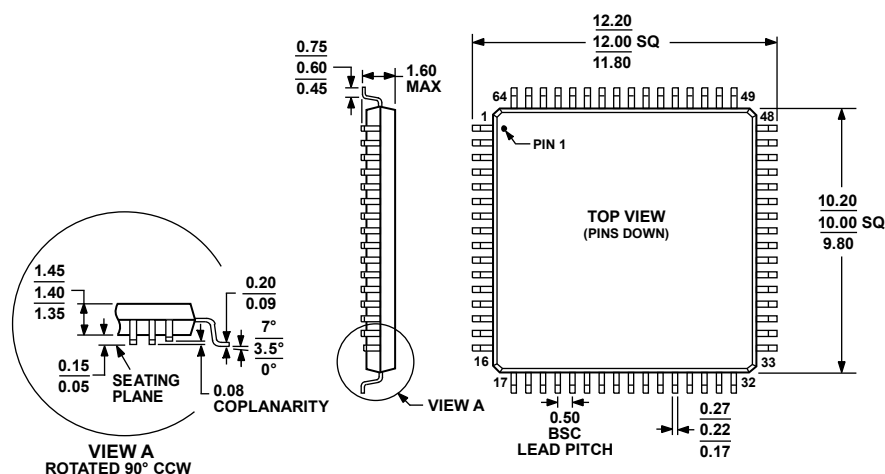
Figure 35. 64-Lead Low Profile Quad Flat Package [LQFP] (ST-64-2) Dimensions shown in millimeters
