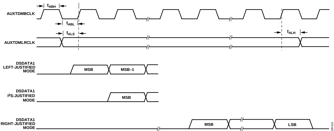
Figure 17. AUCTDM Serial Timing
