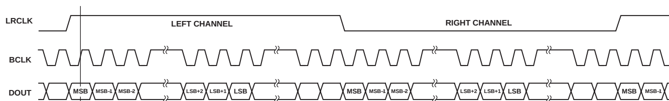
Figure 13. Left-Justified Mode
