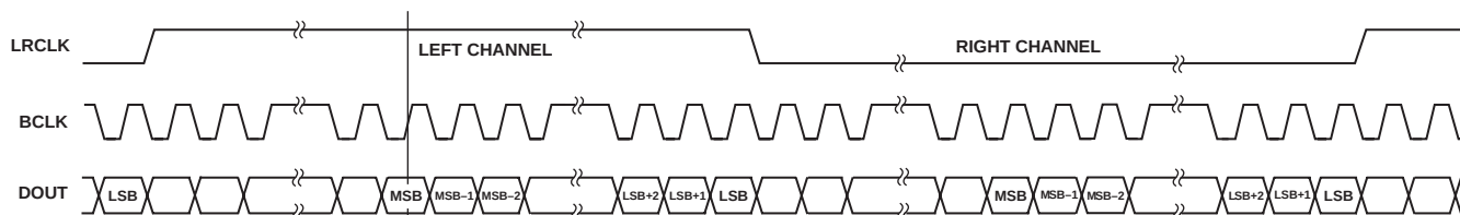
Figure 14. Right-Justified Mode
