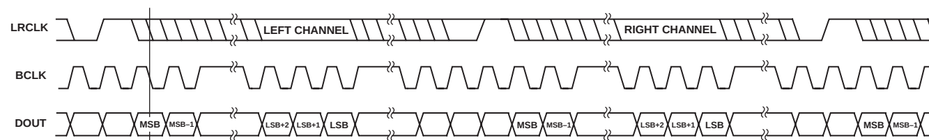
Figure 15. DSP Mode
