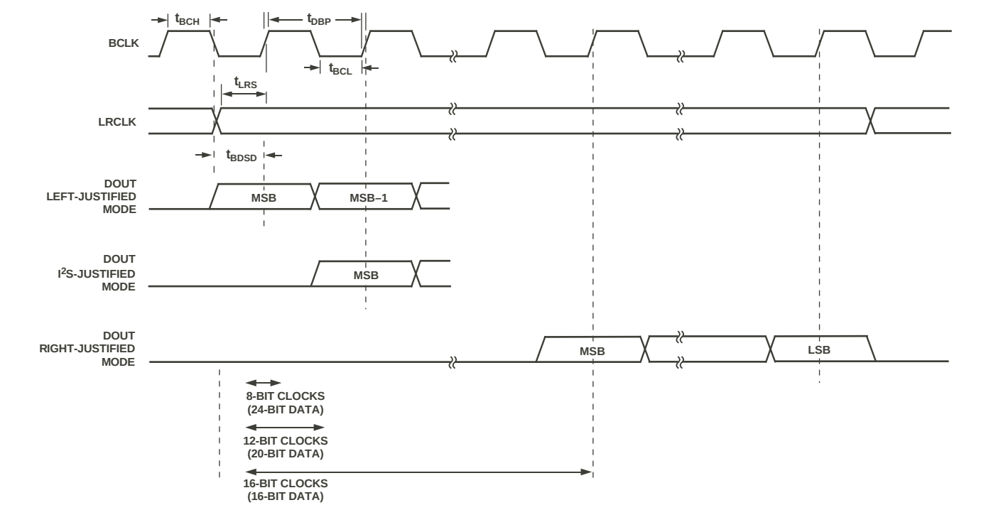
Figure 3. Slave Data Interface Timing
