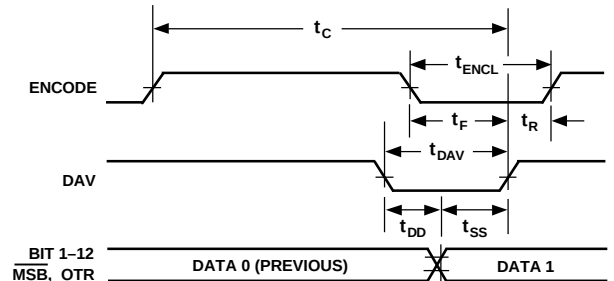
Figure 1b. Encode Pulse LOW
