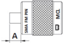
Fig 2. Gaging a Female SMA Connector
