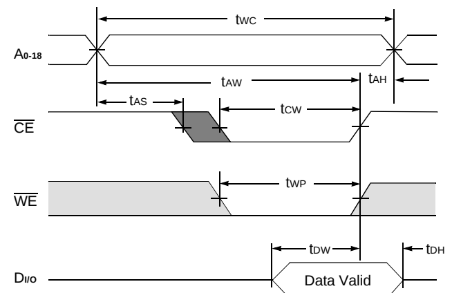
Write Cycle 2 ( \overline{\text{CE}} Controlled, \overline{\text{OE}} = V_{\text{IH}} )
