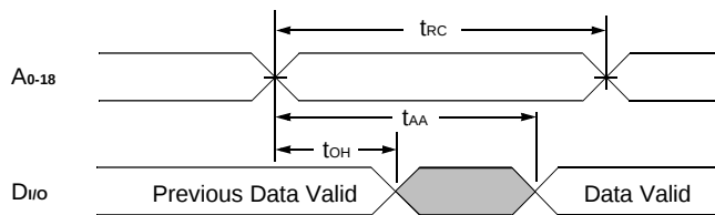
Read Cycle 1 ( \overline{\text{CE}} = \overline{\text{OE}} = \text{V}_{\text{IL}} , \overline{\text{WE}} = \text{V}_{\text{IH}} )
