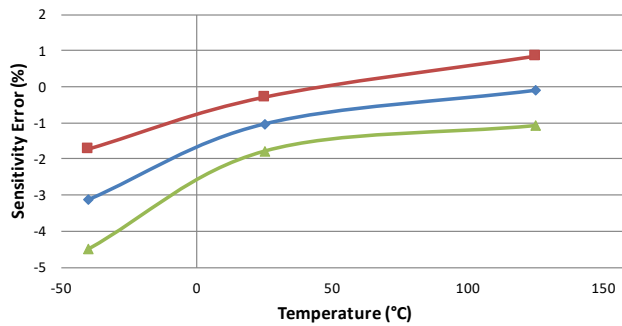
Sensitivity Error vs. Temperature
