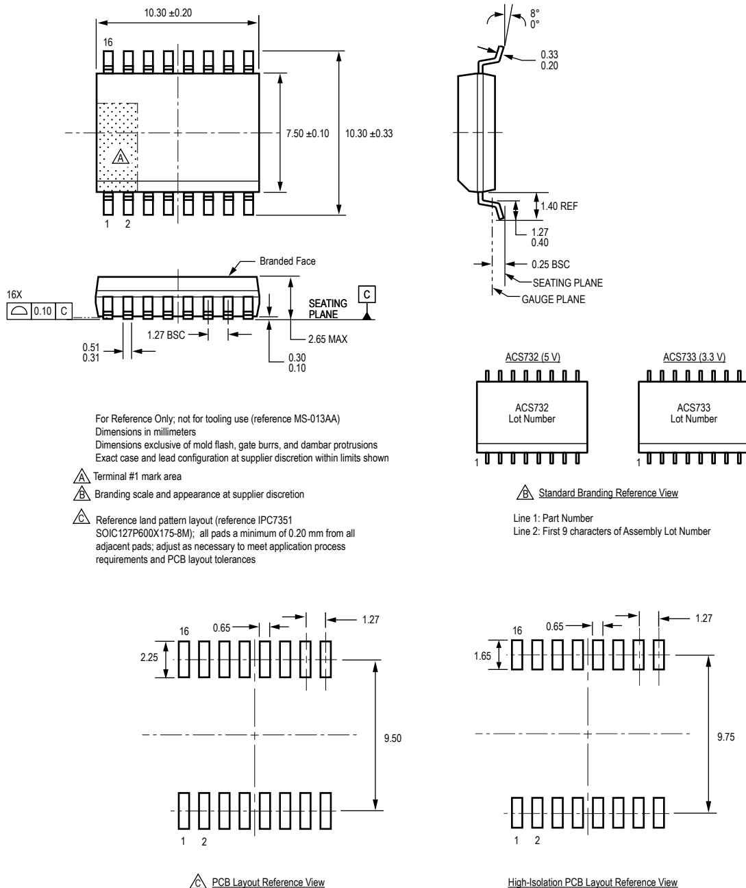
Figure 14: Package LA, 16-Pin SOICW
