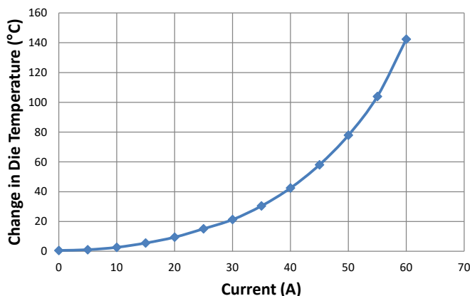
Figure 11: Self Heating in the LA Package Due to Current Flow
