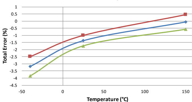
Total Error vs. Temperature
