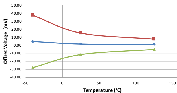
Offset Voltage vs. Temperature
