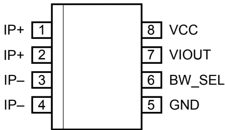
Pin-out Diagram
