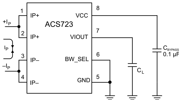
Typical Application
