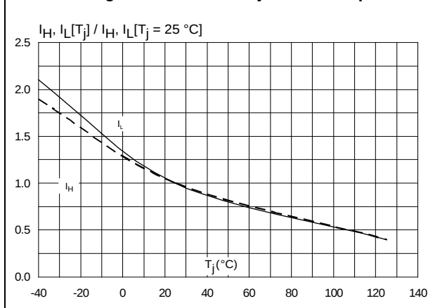
Figure 6: Relative variation of holding current I_H and latching current I_L versus junction temperature
