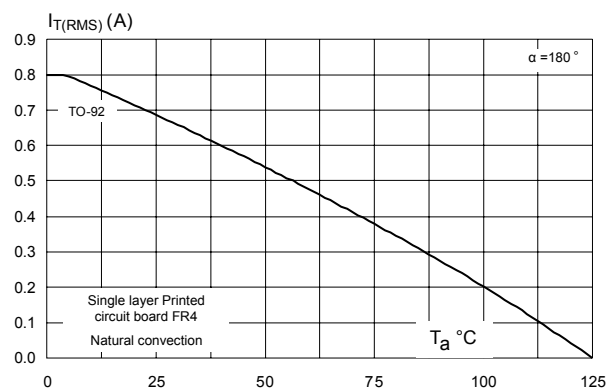
Figure 2. On-state rms current versus ambient temperature
