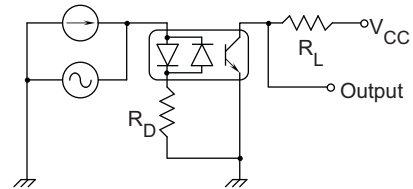
Figure 2. Frequency Response Test Circuit
