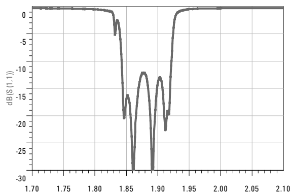
Figure 4. Return Loss [dB] vs. Frequency
