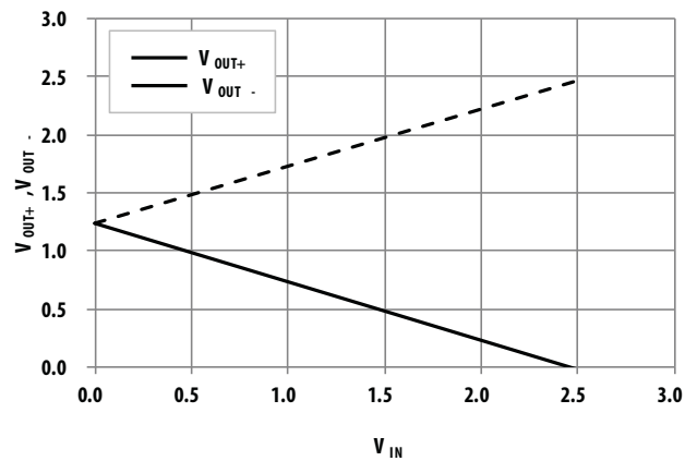
Figure 13 V_{IN} vs. V_{OUT+} , V_{OUT-}
