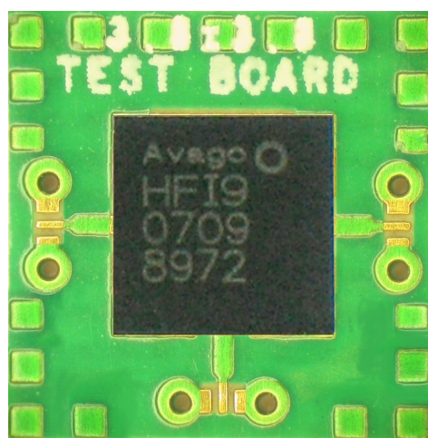
Figure 2. Test circuit with ACMD-7409 duplexer
