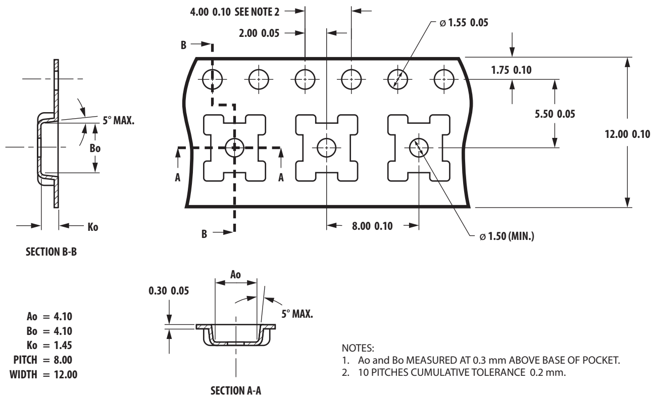
Figure 20. SMD tape packing
