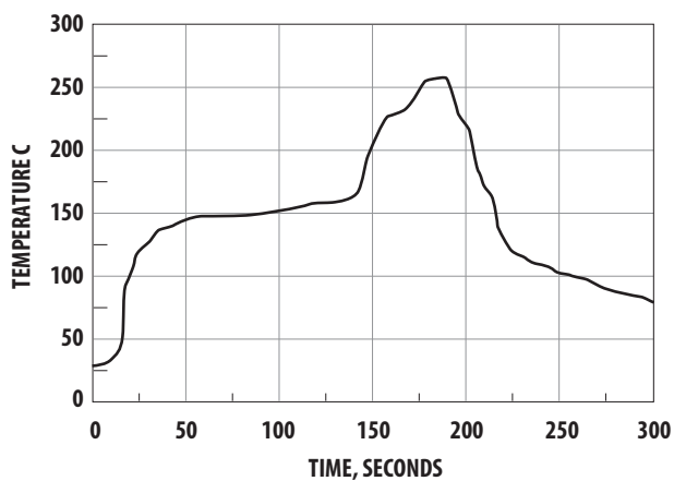
Figure 19. Verified SMT solder profile
