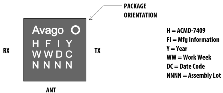
Figure 14. Package marking
