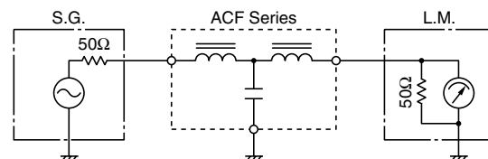
MEASURING CIRCUIT
