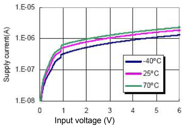
1. Supply current VS. Input Voltage
