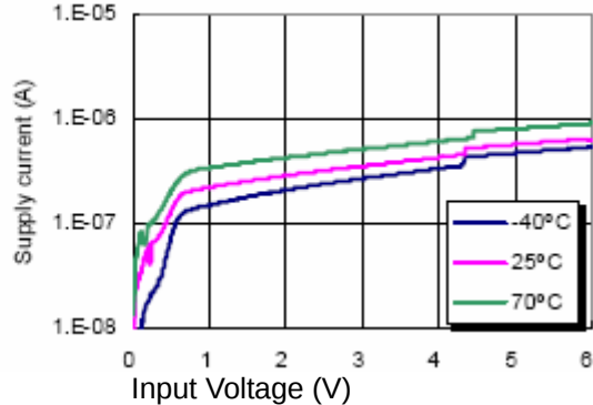
Detector threshold=4.4V
