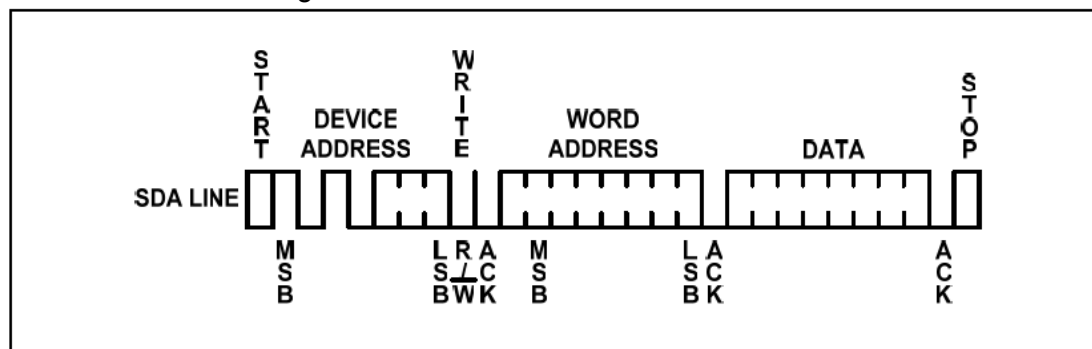
Figure 8 · Byte Write
