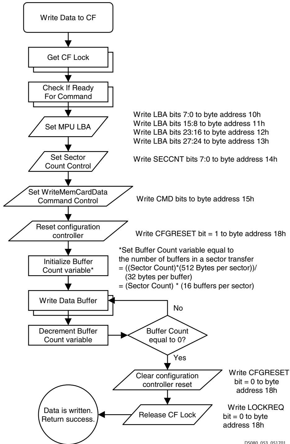
Figure 28: Write Data to CompactFlash Control Flow Process
