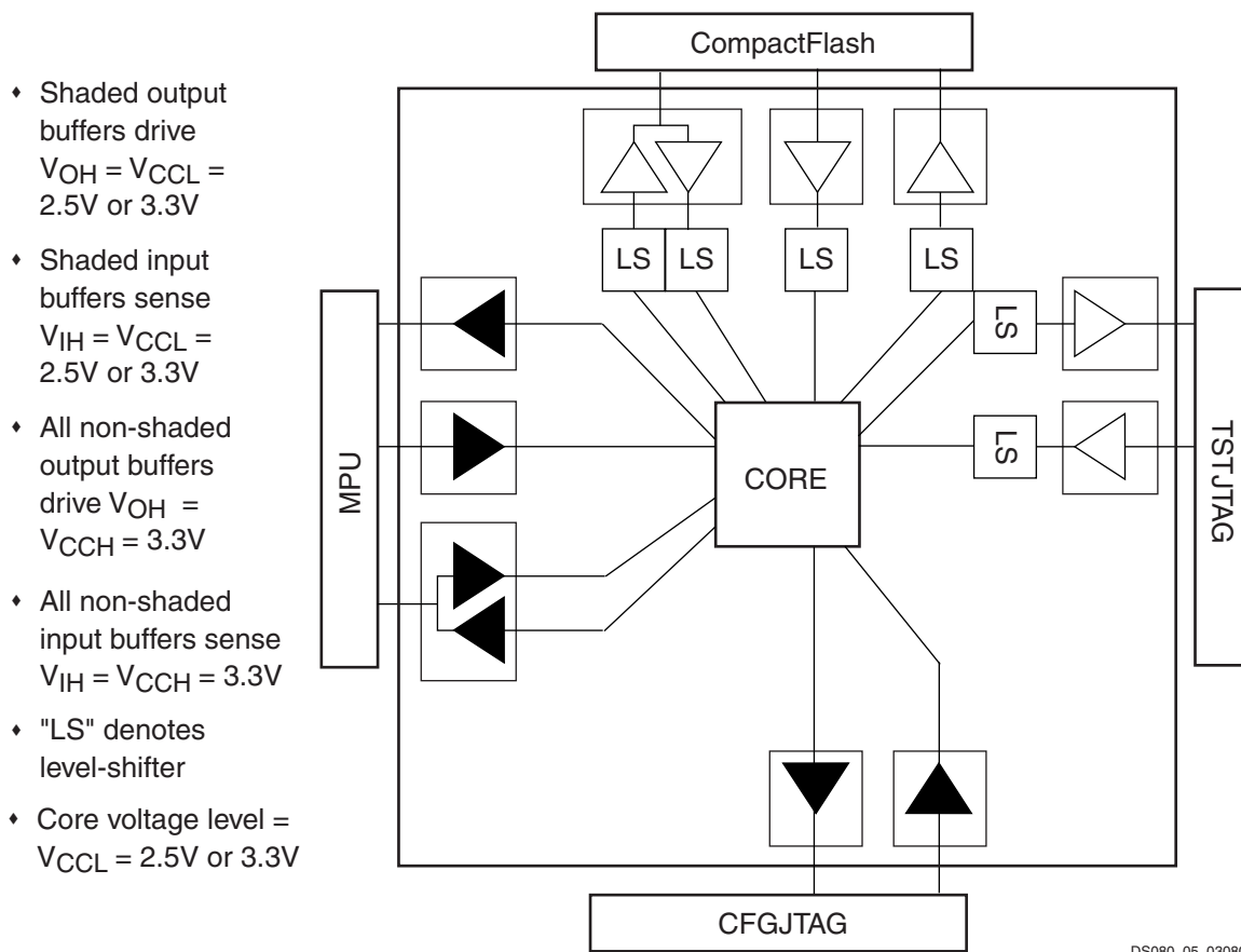
Figure 4: System ACE CF Controller I/O Requirements
