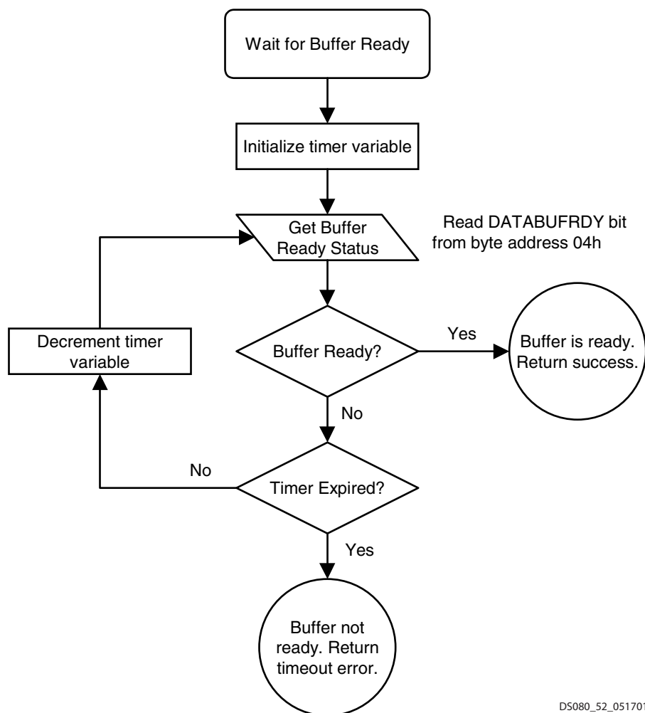
Figure 26: Wait for Buffer Ready Control Flow Process
