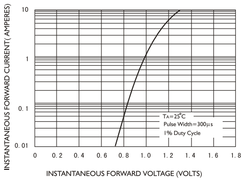
FIG4-TYPICAL FORWARD CHARACTERISTICS
