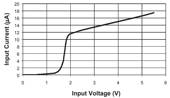
Quiescent Current
