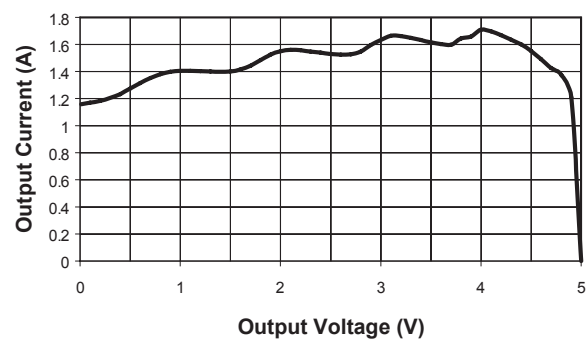
Current Limit
