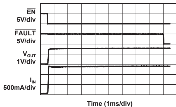
Start Into 1 \Omega Load
